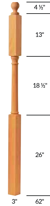
S-4046BT Landing Newel
