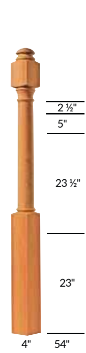
S-4242 Starting Newel
