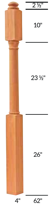
S-4245 Landing Newel
