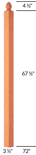
S-4006 Landing Newel
