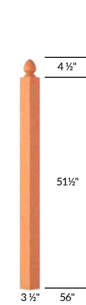
S-4005 Landing Newel
